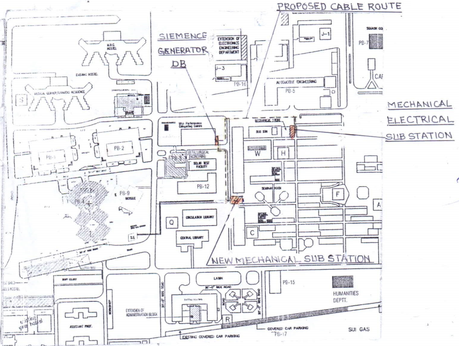
Layout Drawing of proposed cable route
