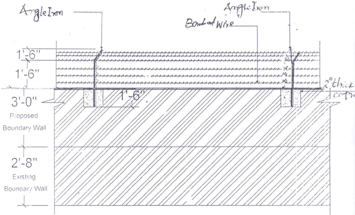
Proposed Boundary Wall Elevation (Typ.)
