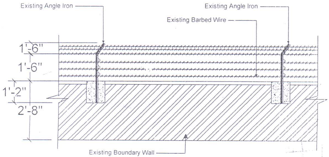
Existing Boundary Wall Elevation (Typ.)
