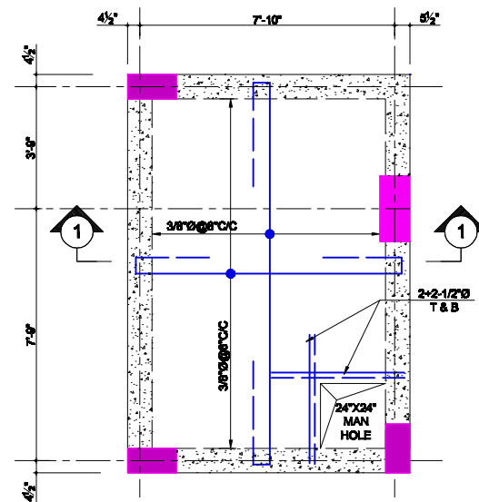
5"-TH. O.H. WATER TANK TOP SLAB
