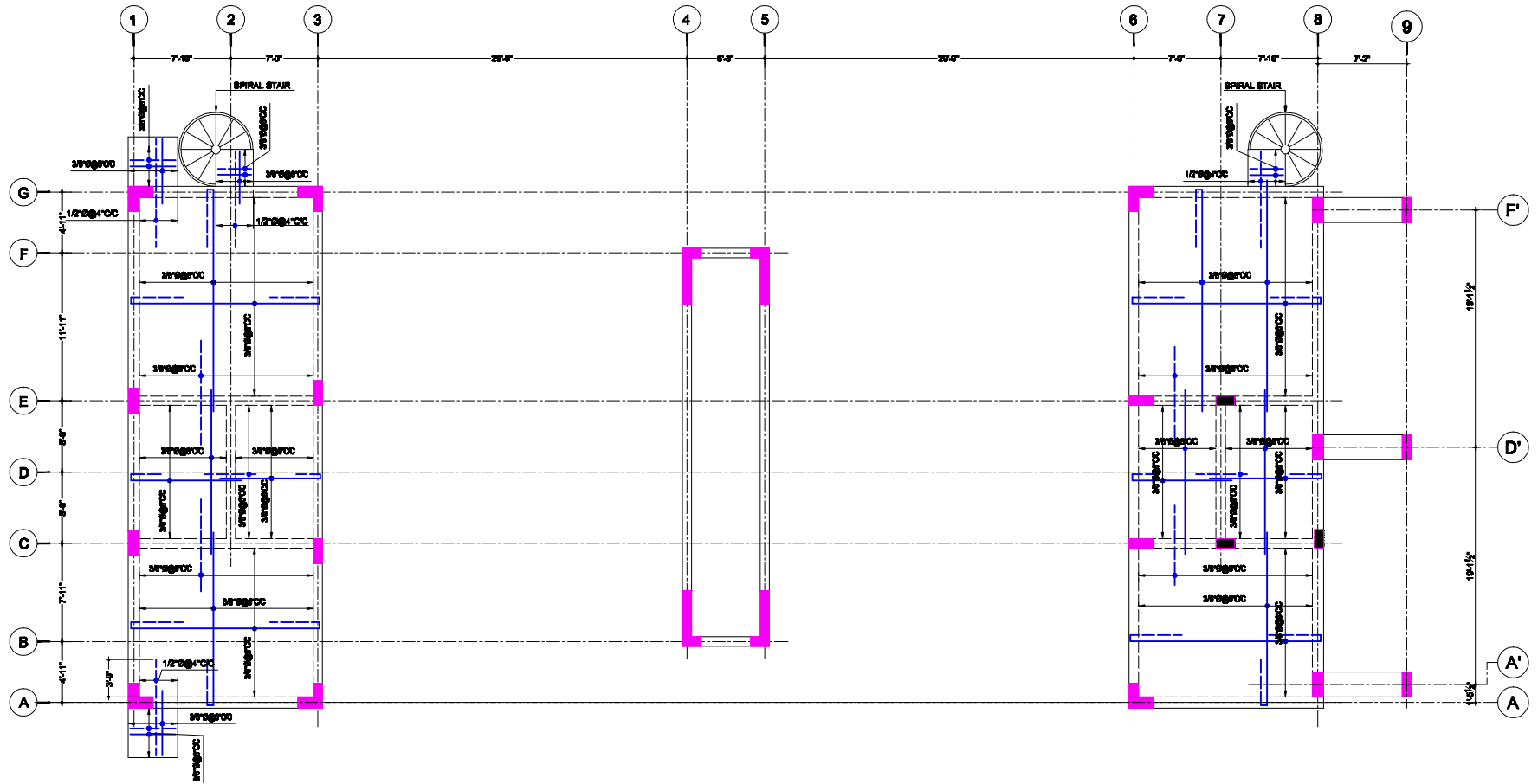
5 TH . GROUND FLOOR SLAB REINF. PLAN AT LEV. +14'-6"
