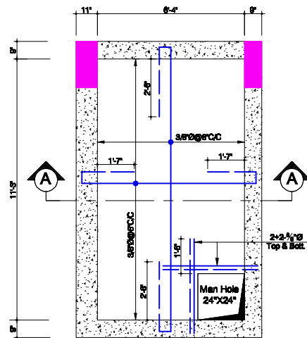
5"-TH. TOP SLAB REINF.PLAN OF U.G.W. TANK
