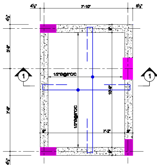
7"-TH. O.H. WATER TANK BOTTOM SLAB
