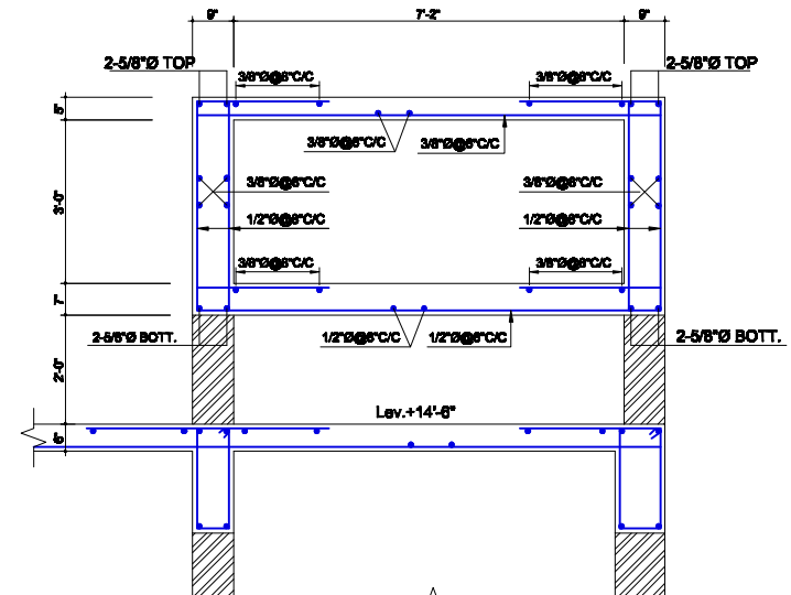
SECTION 1-1
