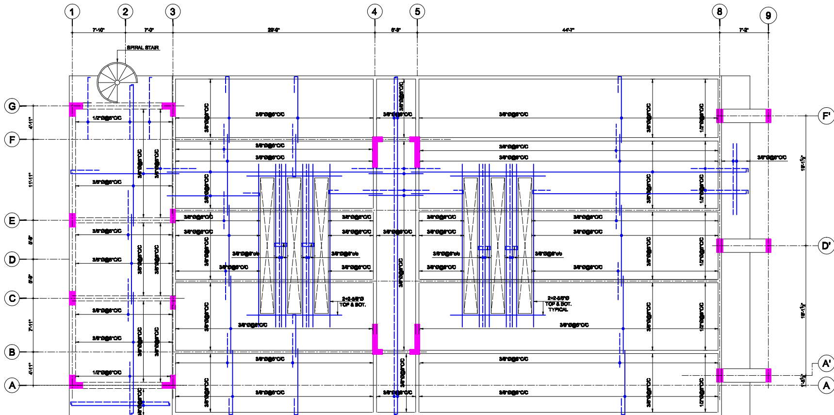
6'-TH. ROOF SLAB REINFORCEMENT PLAN AT LEV. +26'-6"
