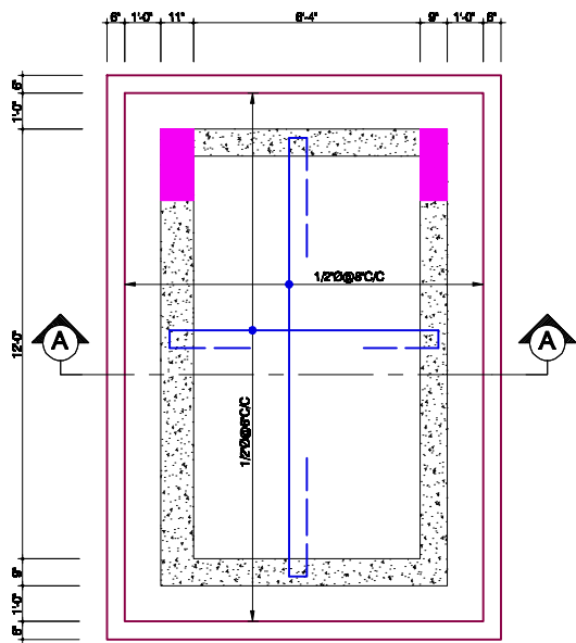
12"-TH. BOTT. SLAB REINF.PLAN OF U.G.W. TANK
