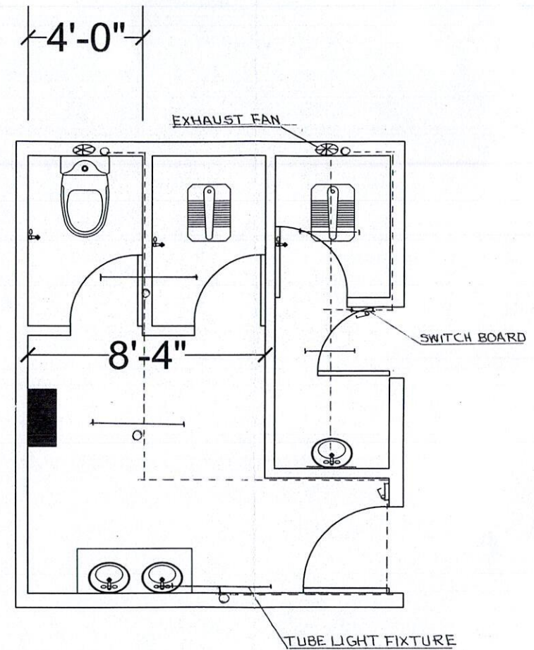
LAYOUT DRAWING OF ELECTRICAL WORKS .
