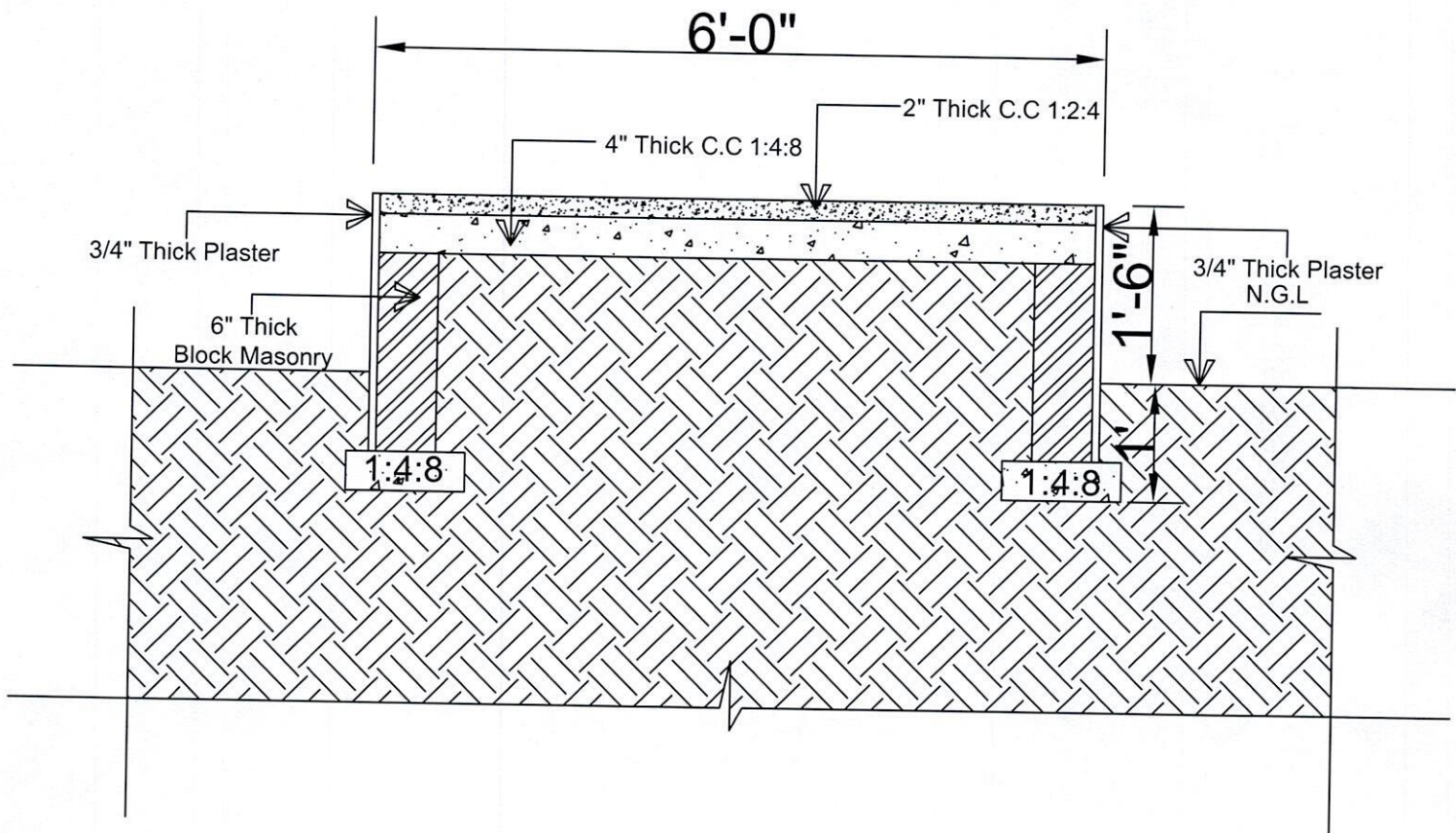
TYPICAL SECTION OF WALK WAY
