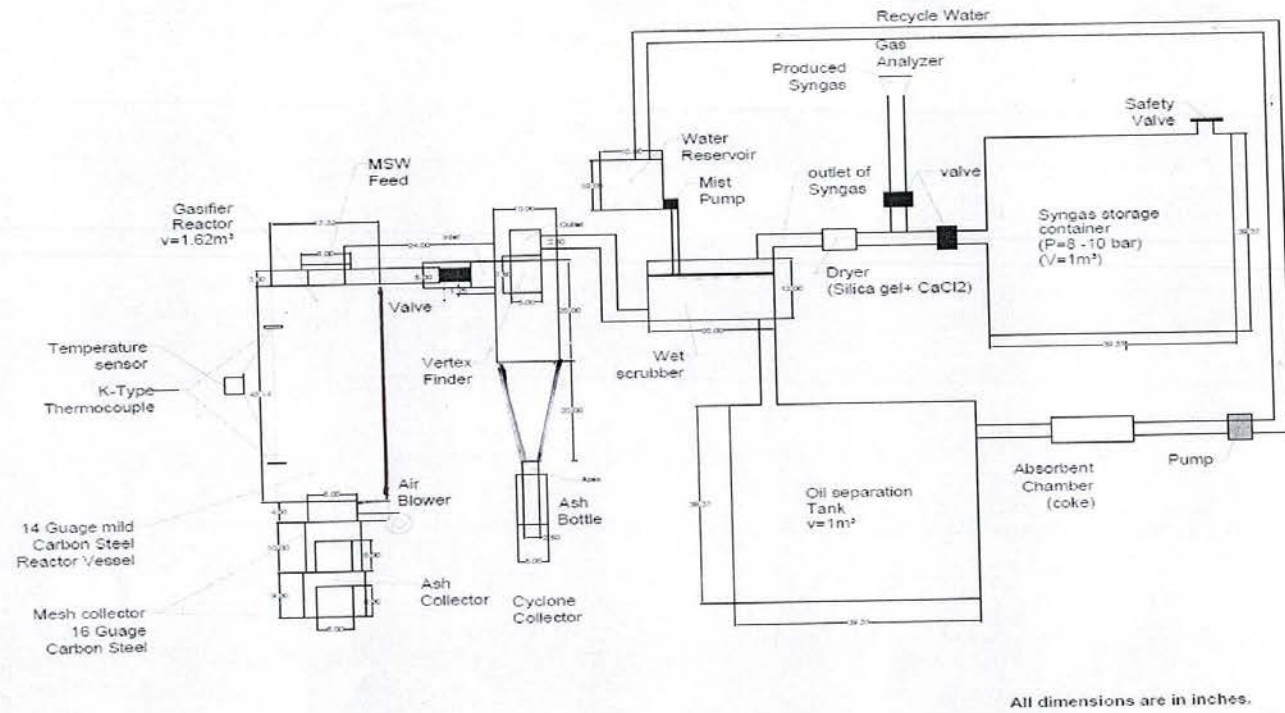
Schematic diagram of an updraft MSW gasifier
