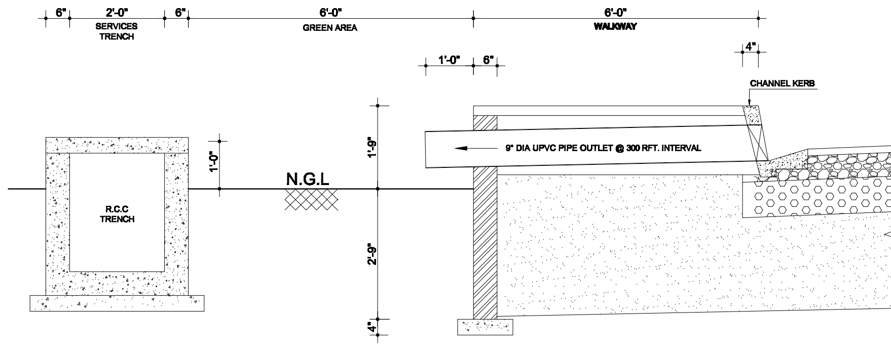
TYPICAL DETAIL OF RAIN WATER OUTLET-2
