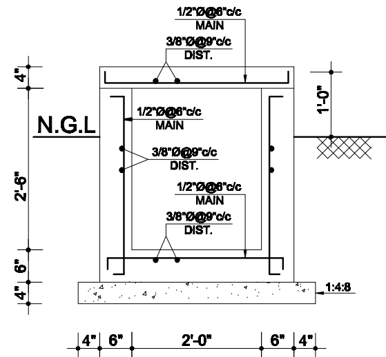
REINF. DETAIL OF SERVICES TRENCH
