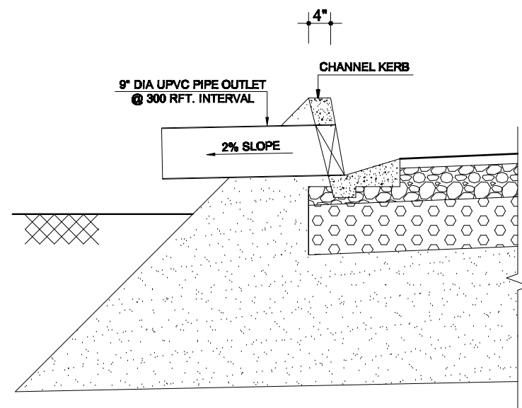
TYPICAL DETAIL OF RAIN WATER OUTLET-1
