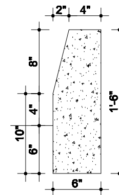
KERB STONE
