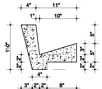
CHANNEL KERB
