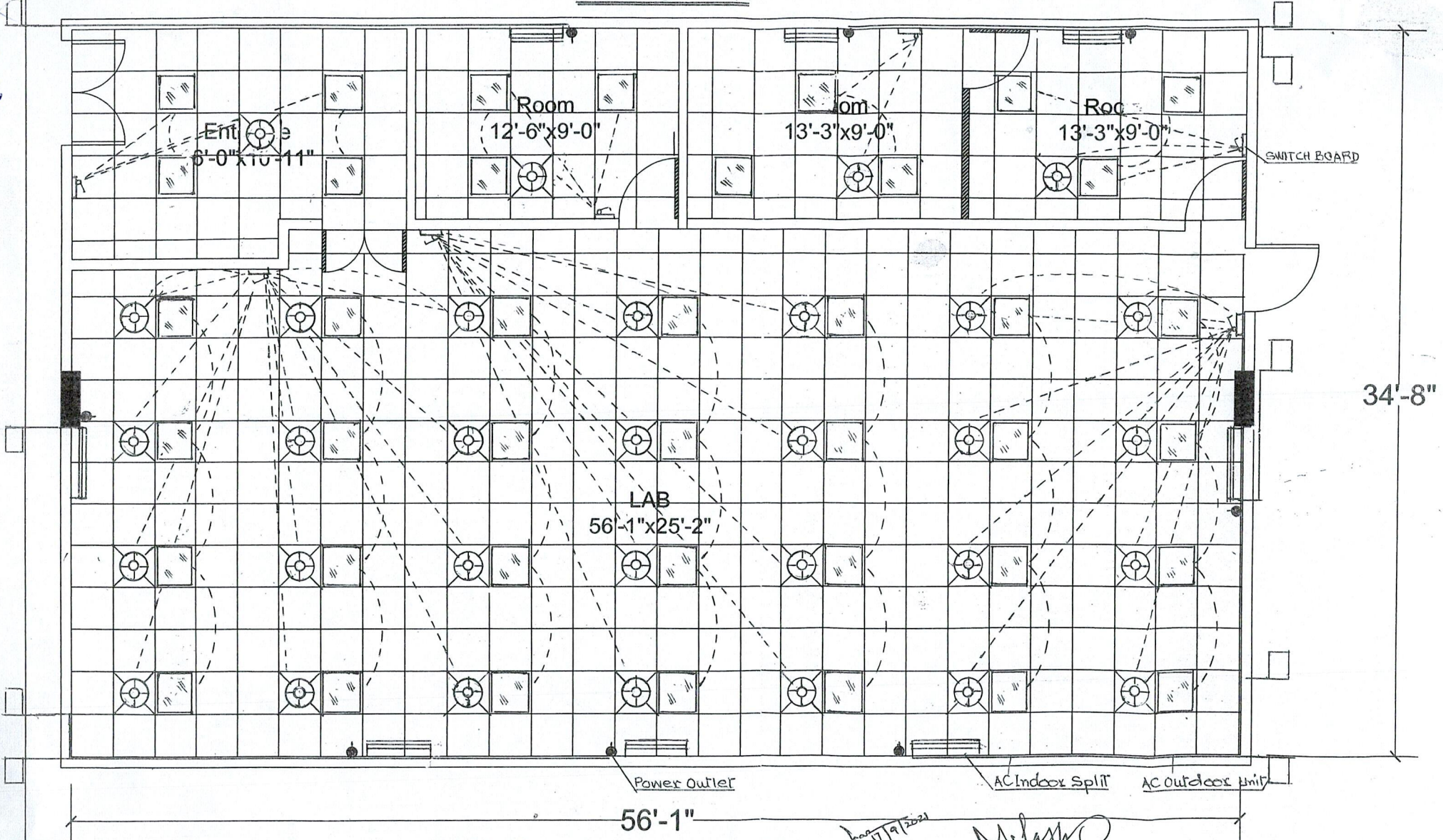
LAYOUT DRAWING OF ELECTRICAL WORK
