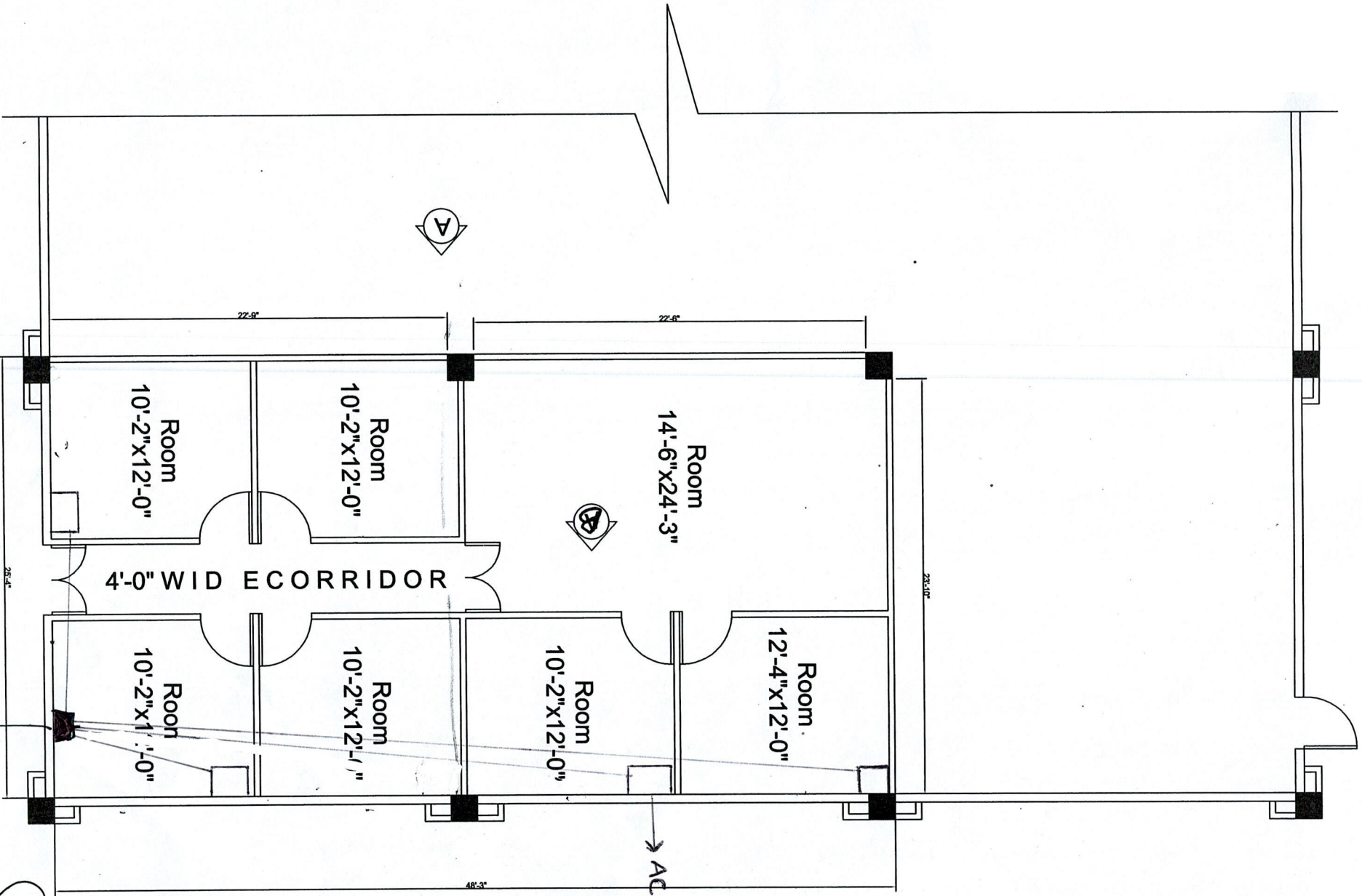
PROPOSED ALUMINUM PARTITION PLAN
