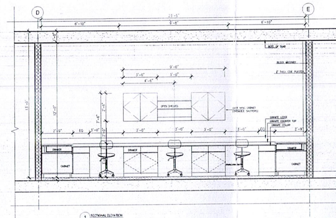
1 SECTIONAL ELEVATION Scale: 1/4" = 1'-0"
