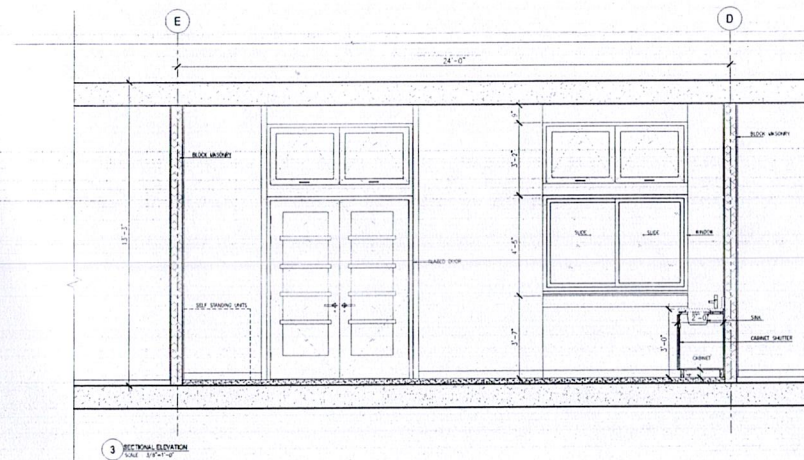
3 SECTIONAL ELEVATION Scale: 1/4" = 1'-0"
