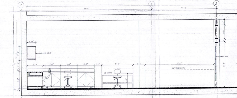
4 SECTIONAL ELEVATION Scale: 1/4" = 1'-0"
