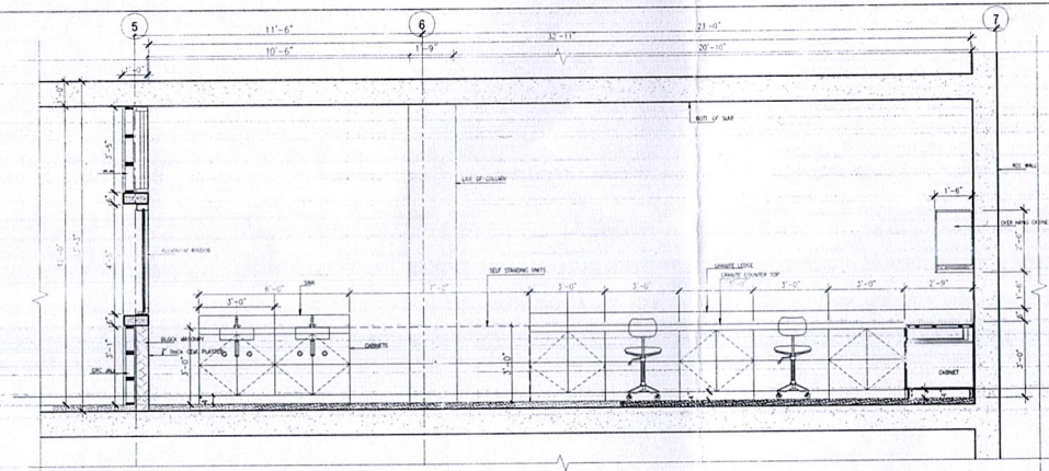
2 SECTIONAL ELEVATION Scale: 1/4" = 1'-0"
