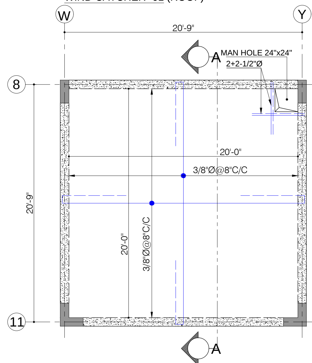
5"TH. O.H.W. TANK TOP SLAB REINF. PLAN
