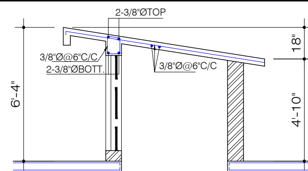
DETAIL OF WIND CATCHER -01
