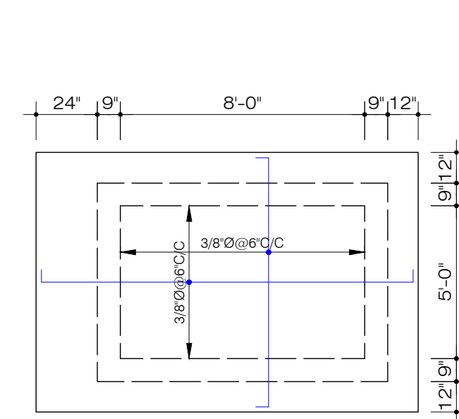
PLAN OF WIND CATCHER -02 (ROOF)
