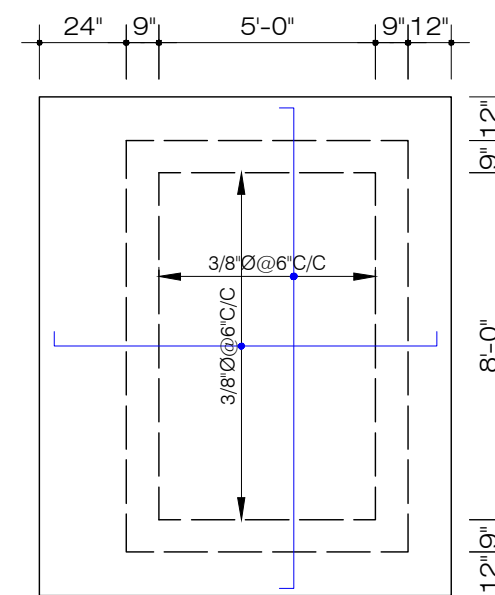
PLAN OF WIND CATCHER -01 (ROOF)
