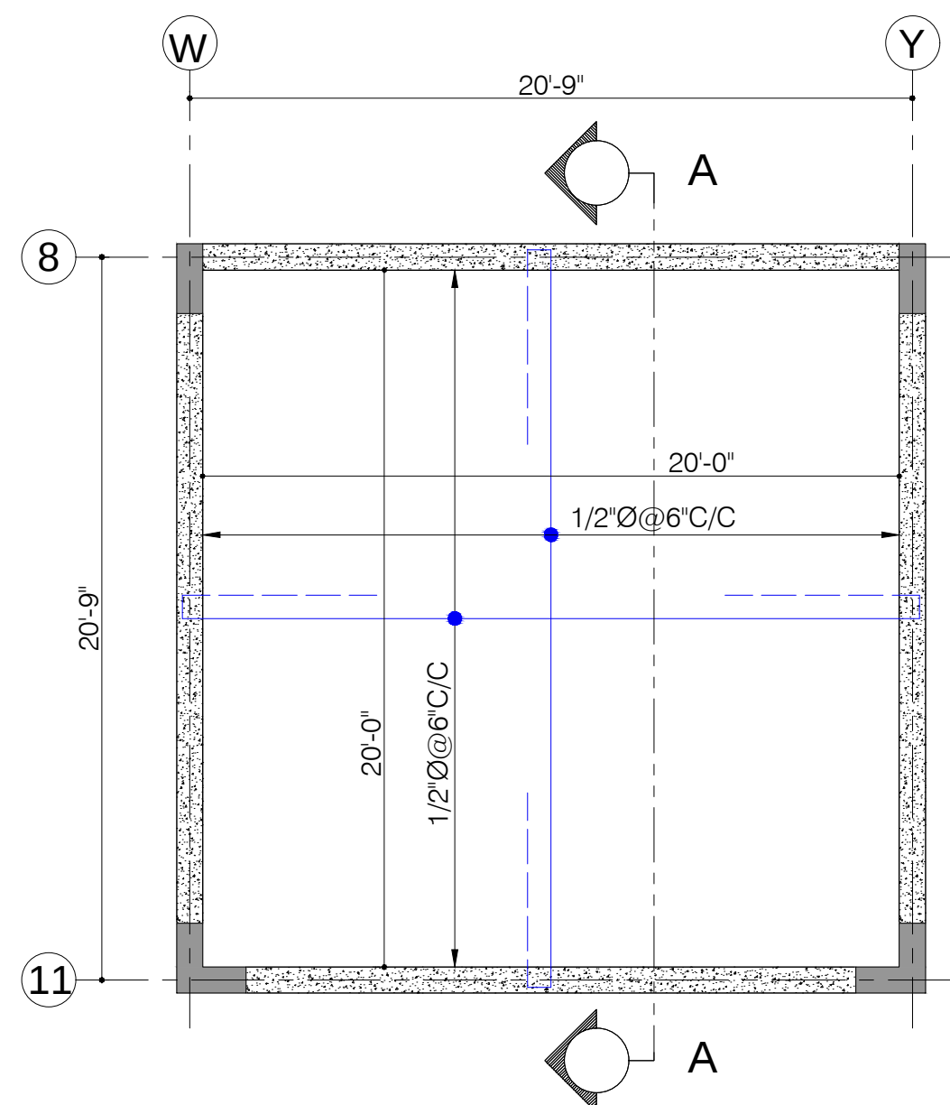
8"TH. O.H.W. TANK BOTTOM SLAB REINF. PLAN
