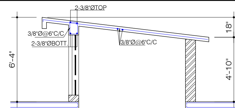
DETAIL OF WIND CATCHER -02
