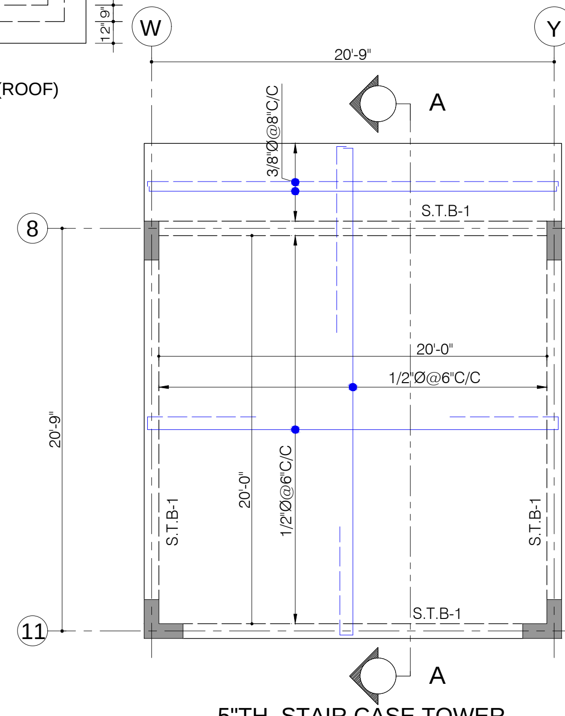
5"TH. STAIR CASE TOWER SLAB REINF. PLAN LEV. 37'-6"
