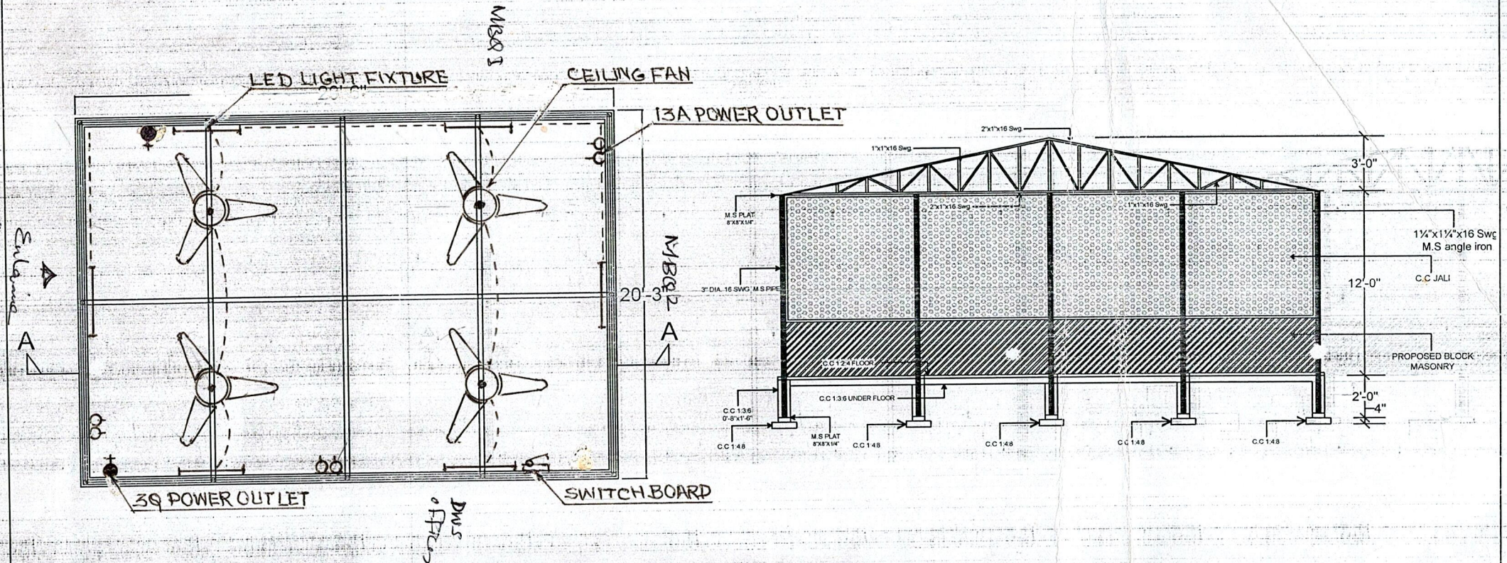
LAYOUT DRAWING OF LIGHT, FAN AND POWER OUTLET
