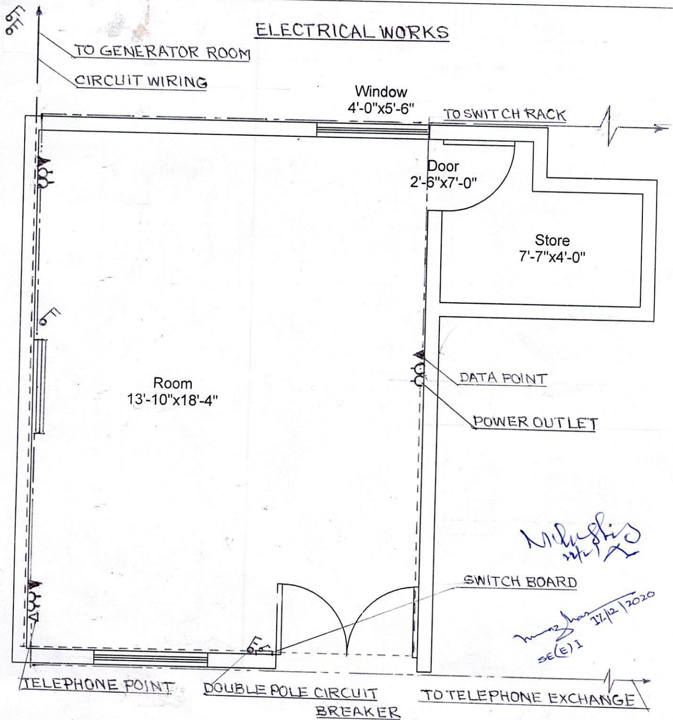
LAYOUT DRAWING OF POWER OUTLET, DATA POINT, TELEPHONE POINT & AC UNIT.
