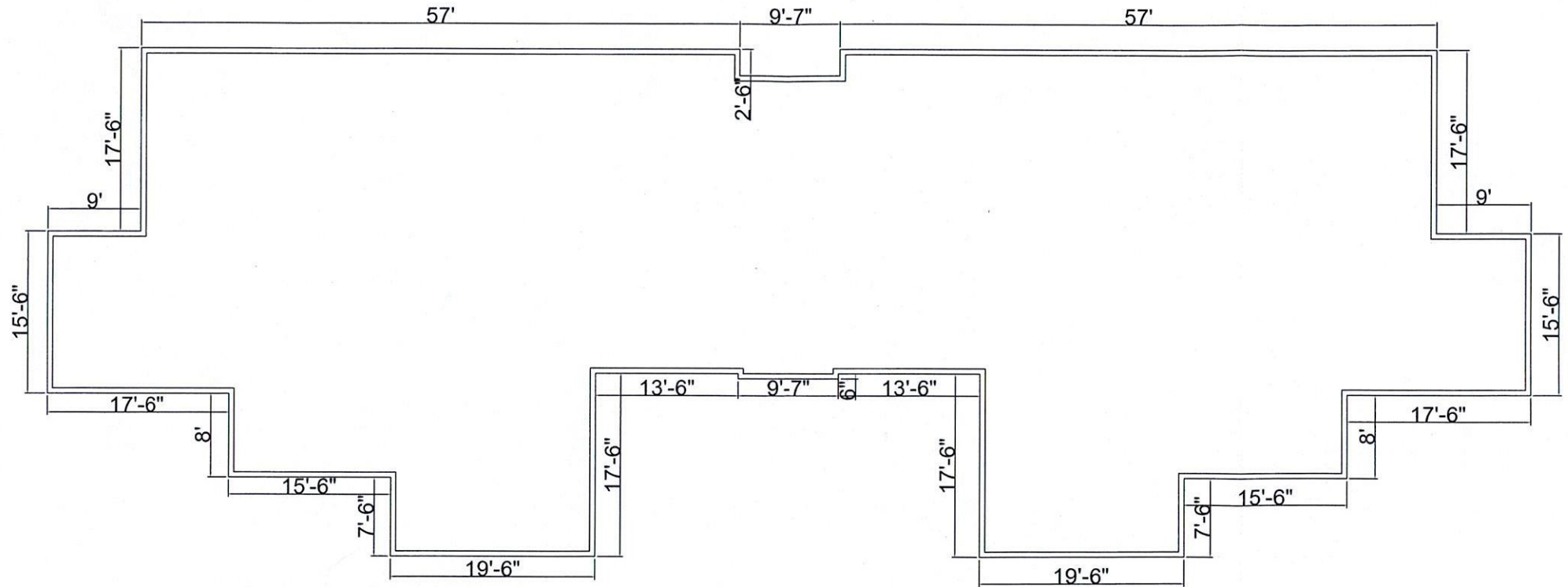
Roof Plan of Staff Resident Block A-01 to A-04
